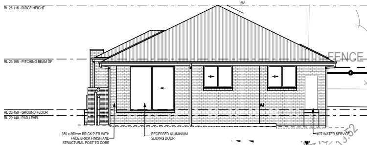
SOUTH ELEVATION
